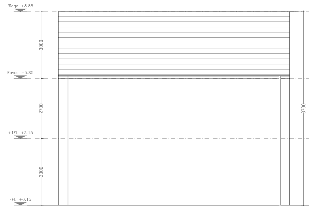
House Type N2 End of Terrace Side Elevation
