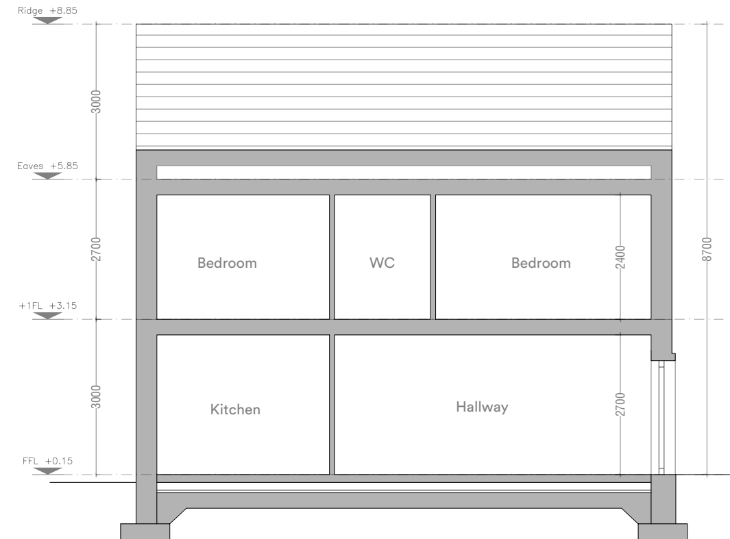
House Type N2 End of Terrace Section A.A
